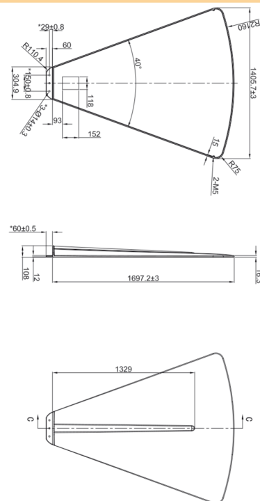
Figure 2. Dimension of solar
